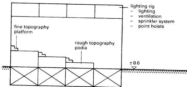
③ Lifting stages - sketch showing principles
